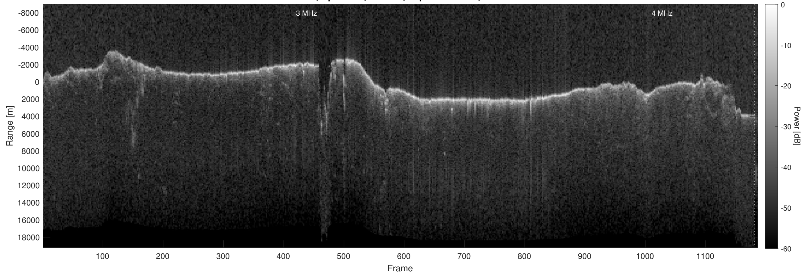
Orbit 6126, Optimized, Window, Depth-Corrected, Channel 2
