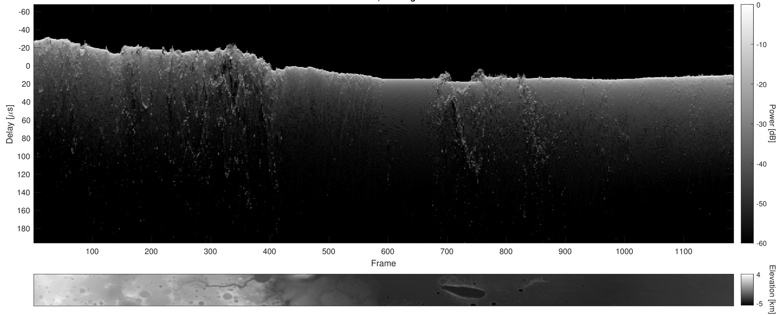
Orbit 6127, Cluttergram
