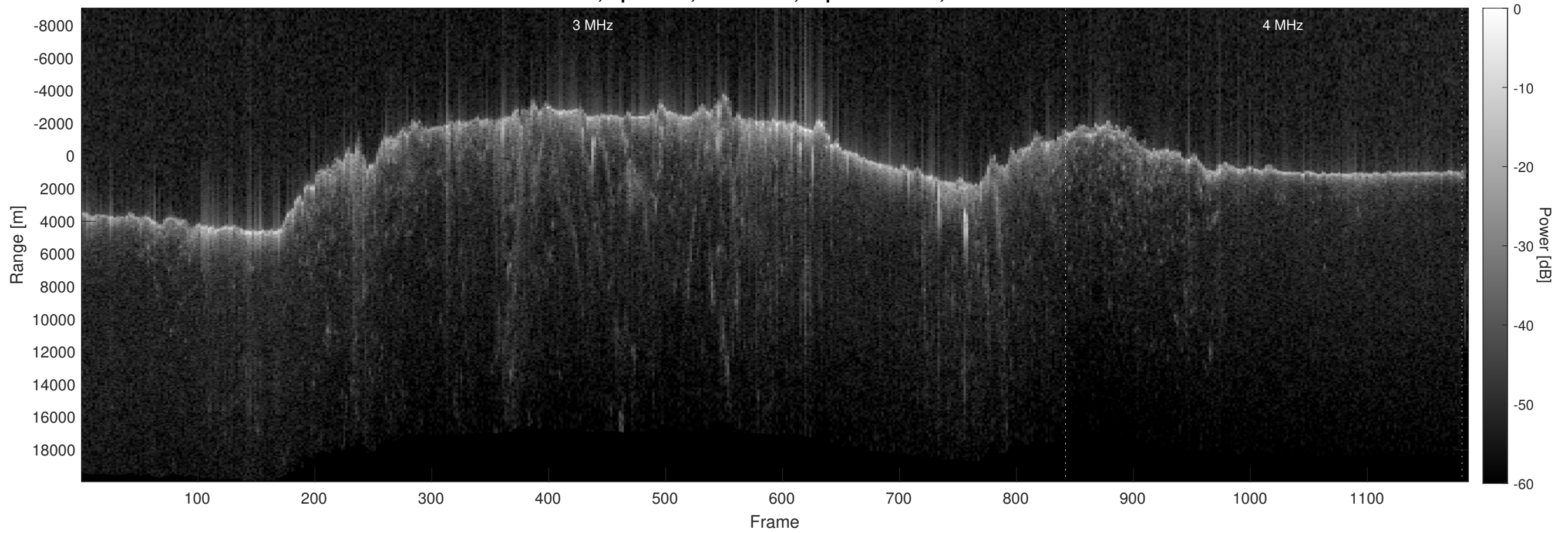
Orbit 6128, Optimized, No Window, Depth-Corrected, Channel 2
