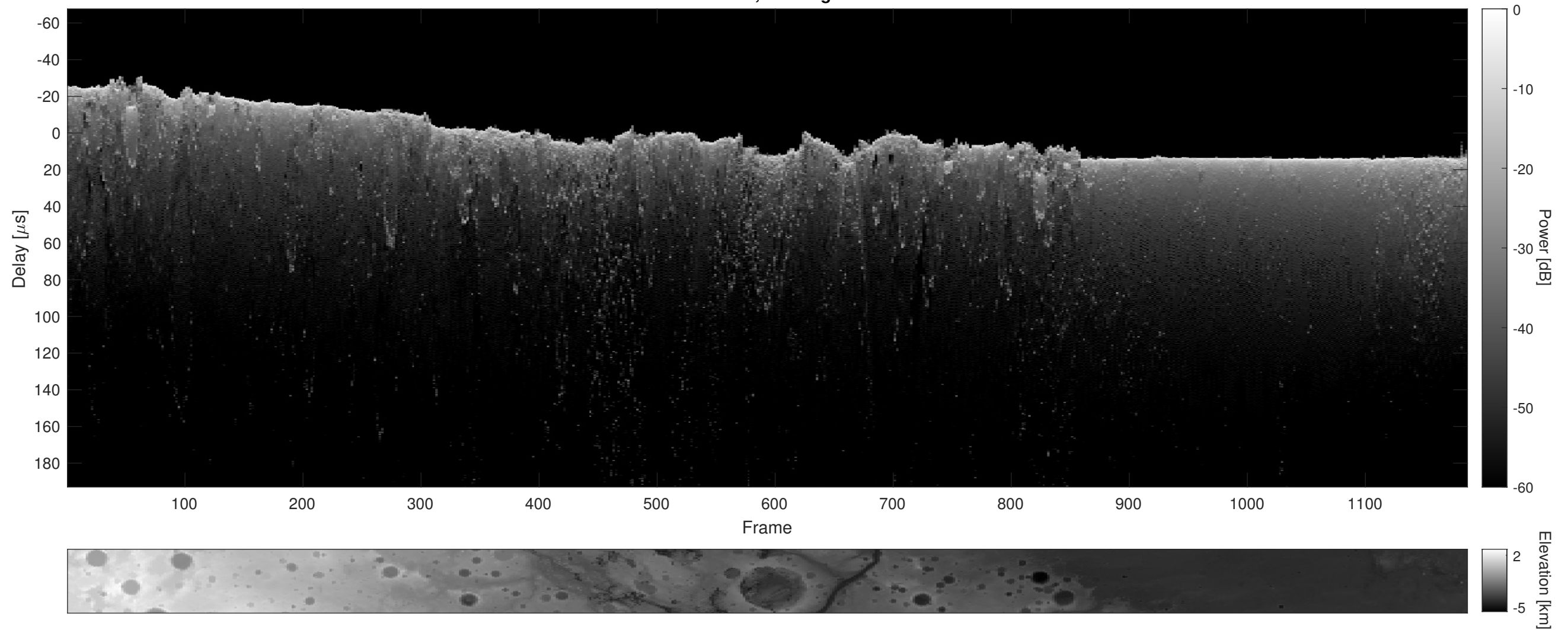
Orbit 6129, Cluttergram
