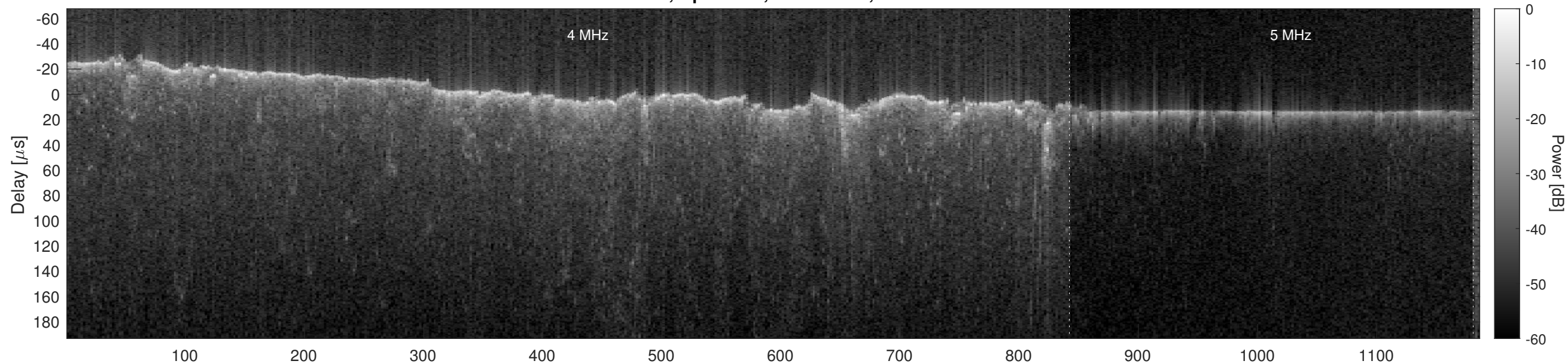
Orbit 6129, Optimized, No Window, Channel 2
