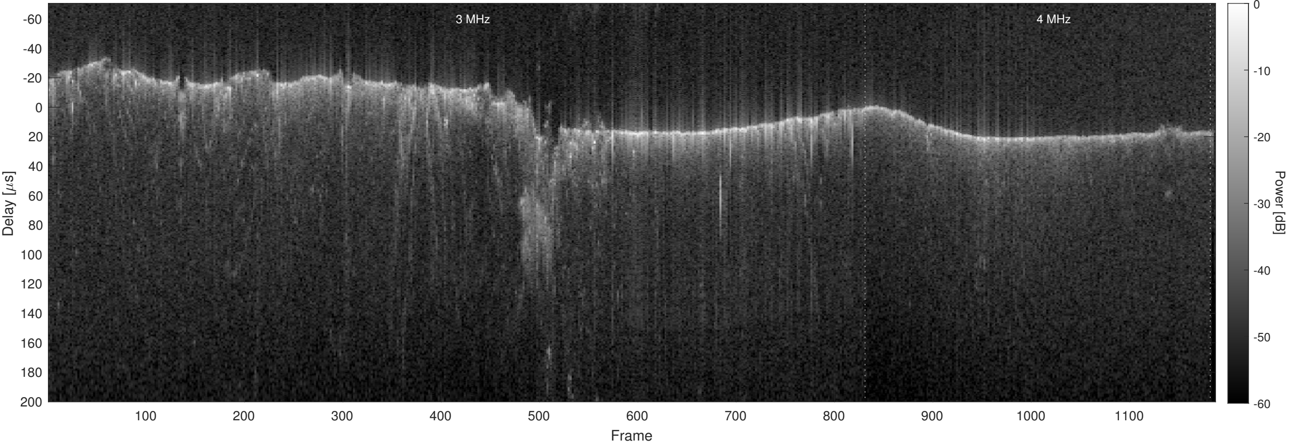
Orbit 6131, Optimized, No Window, Channel 2
