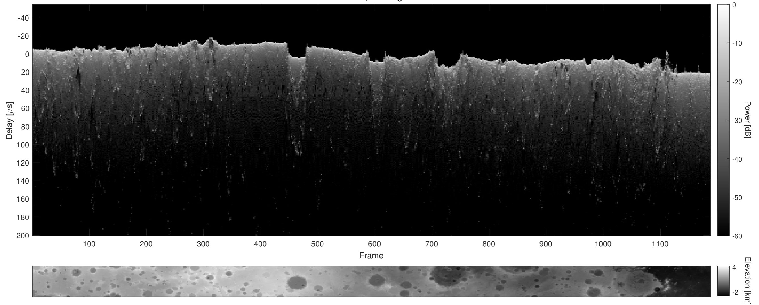
Orbit 6132, Cluttergram
