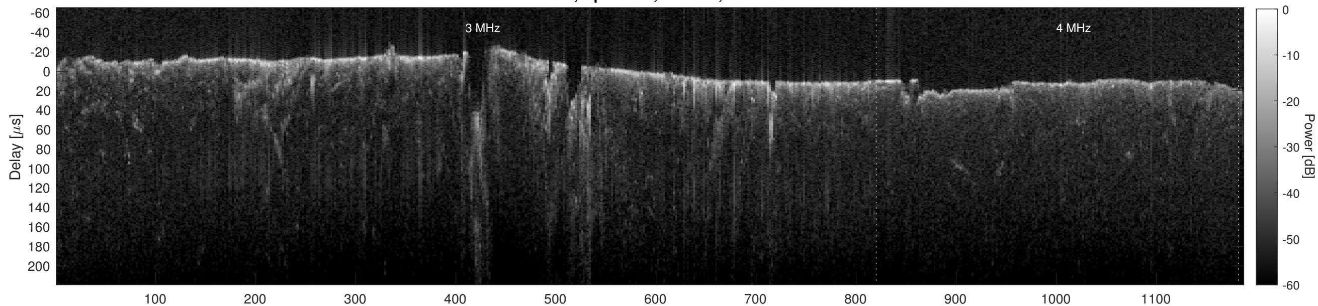
Orbit 6133, Cluttergram
