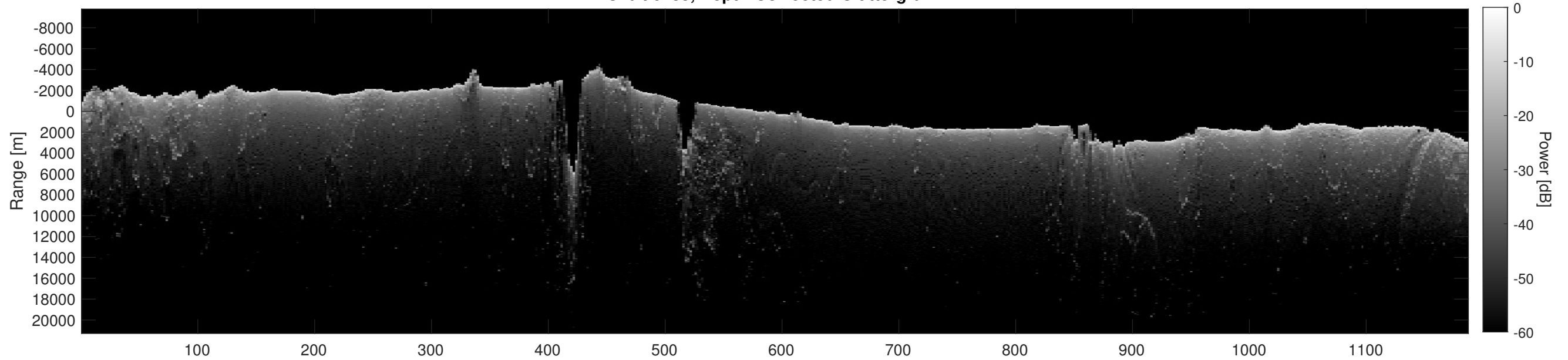
Orbit 6133, Depth-Corrected Cluttergram
