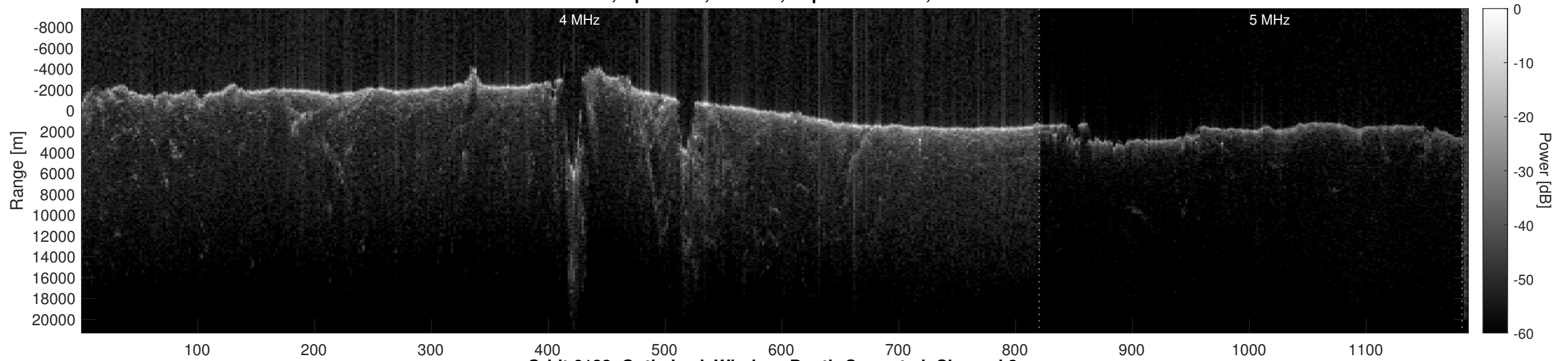
Orbit 6133, Optimized, Window, Depth-Corrected, Channel 2
