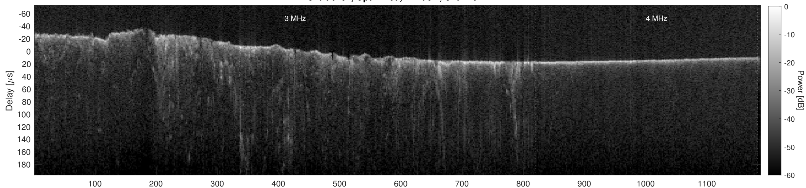
Orbit 6134, Cluttergram
