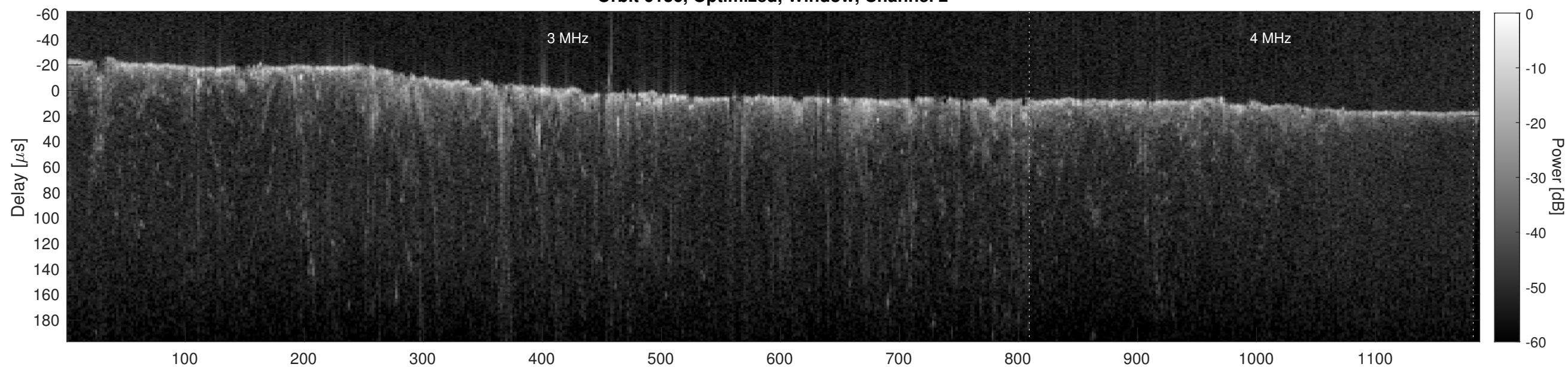
Orbit 6136, Cluttergram
