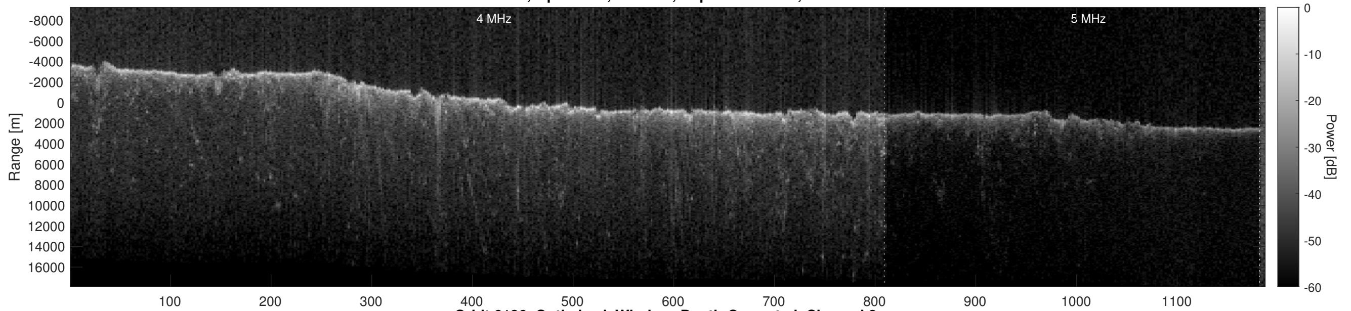
Orbit 6136, Optimized, Window, Depth-Corrected, Channel 2
