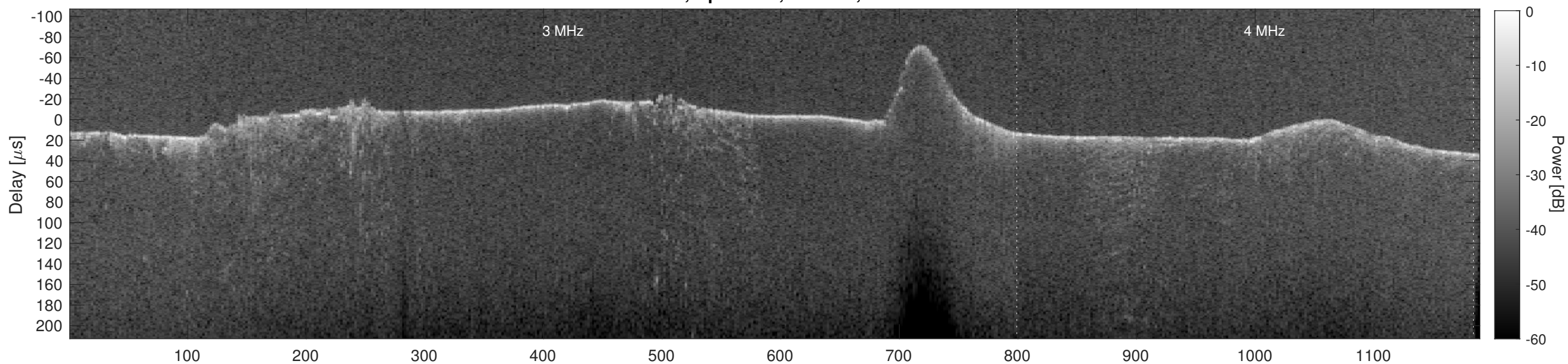
Orbit 6137, Cluttergram
