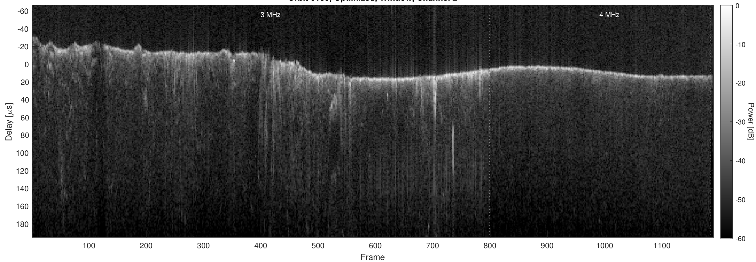
Orbit 6138, Optimized, Window, Channel 2
