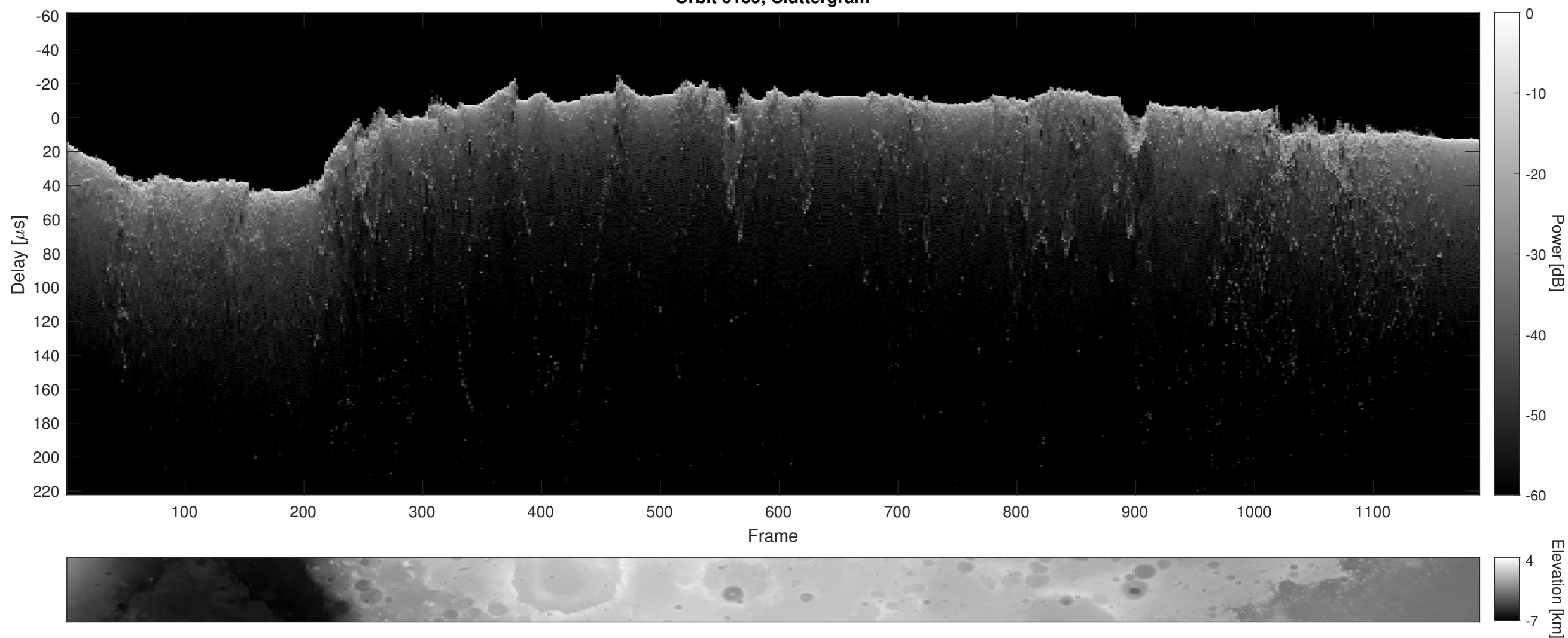
Orbit 6139, Cluttergram
