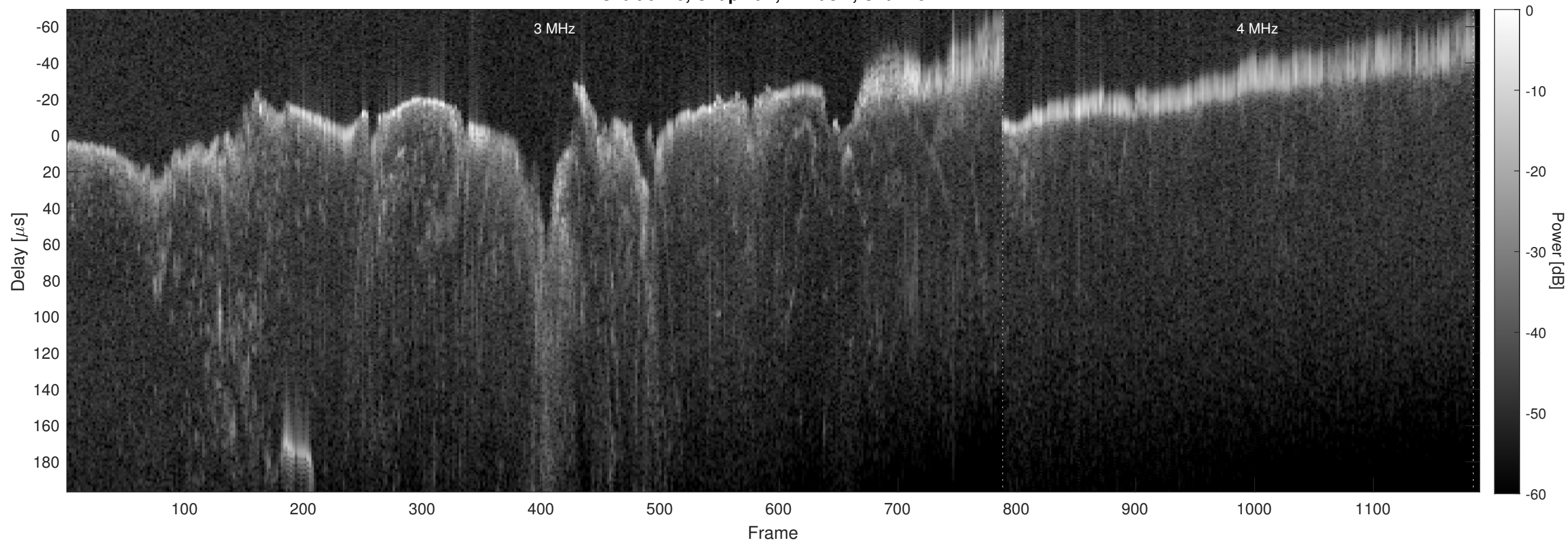
Orbit 6140, Chapman, Window, Channel 2
