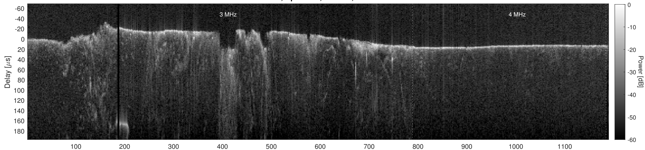
Orbit 6140, Cluttergram
