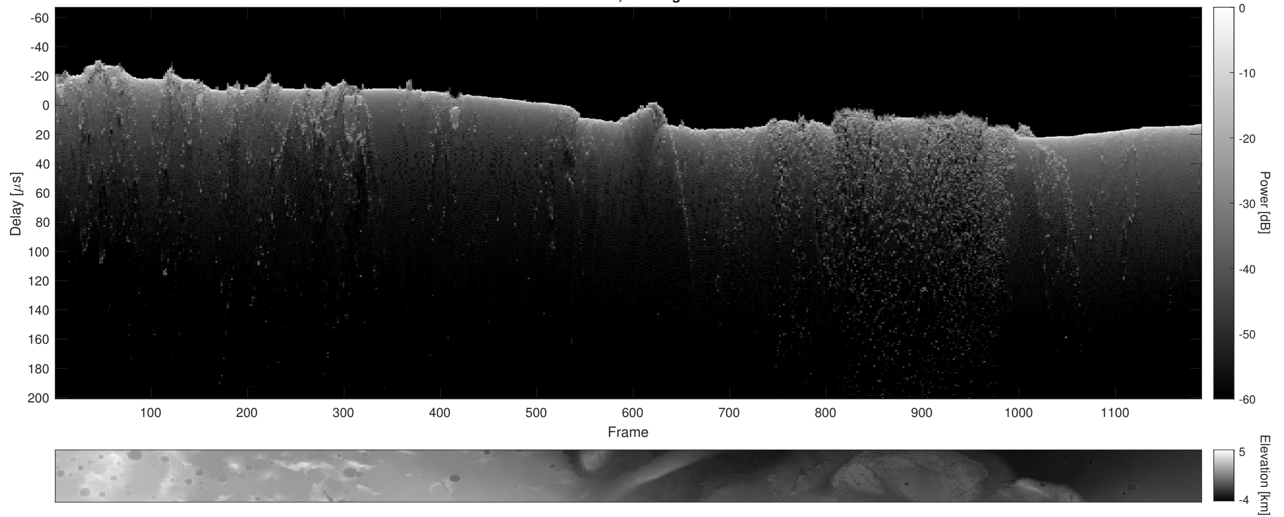
Orbit 6141, Cluttergram
