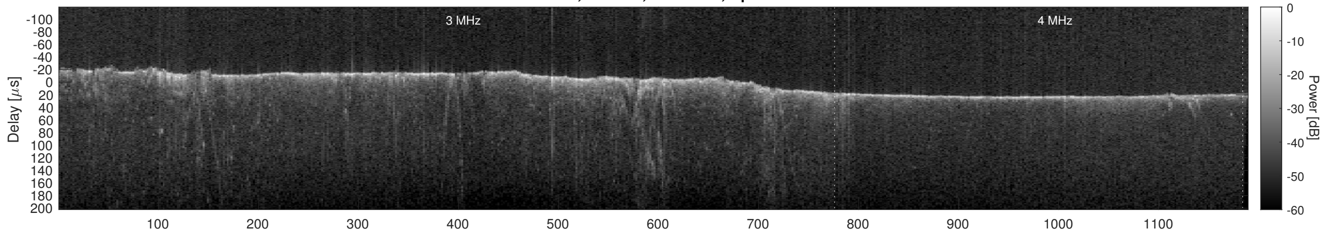
Orbit 6142, Cluttergram
