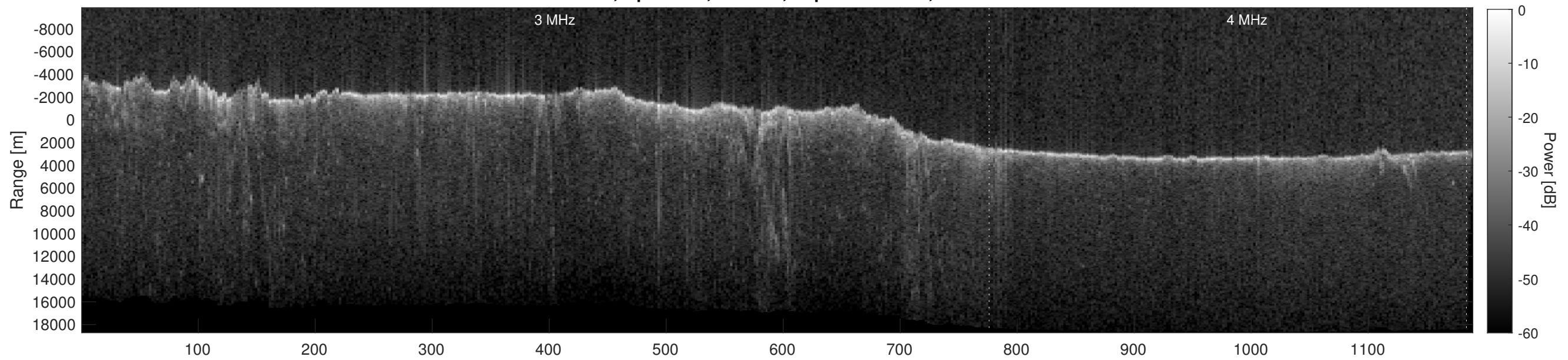
Orbit 6142, Depth-Corrected Cluttergram
