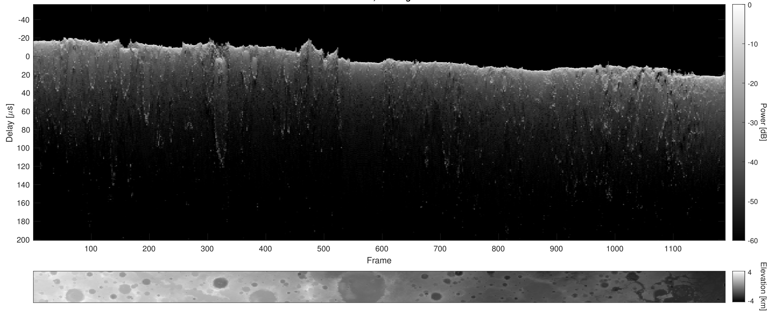
Orbit 6143, Cluttergram
