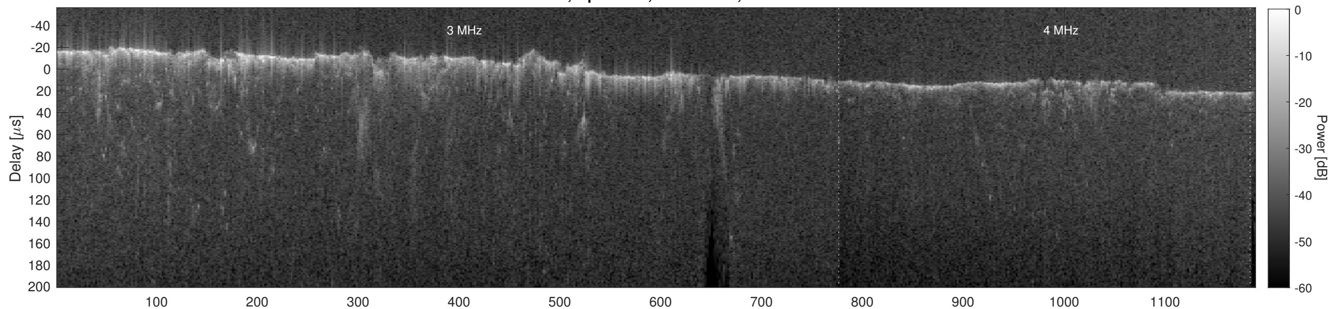
Orbit 6143, Cluttergram
