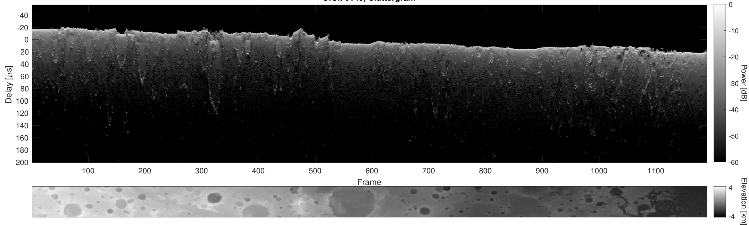
Orbit 6143, Cluttergram
