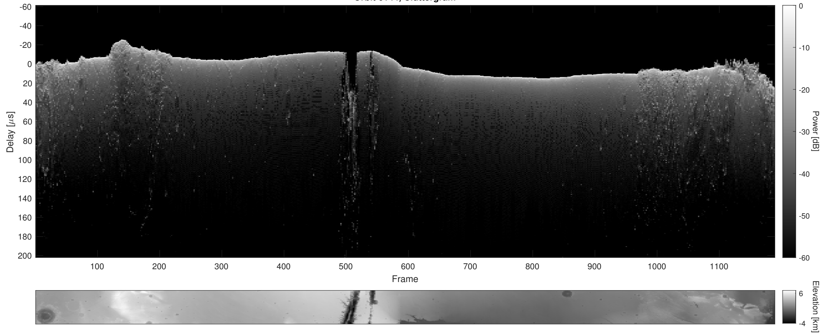
Orbit 6144, Cluttergram
