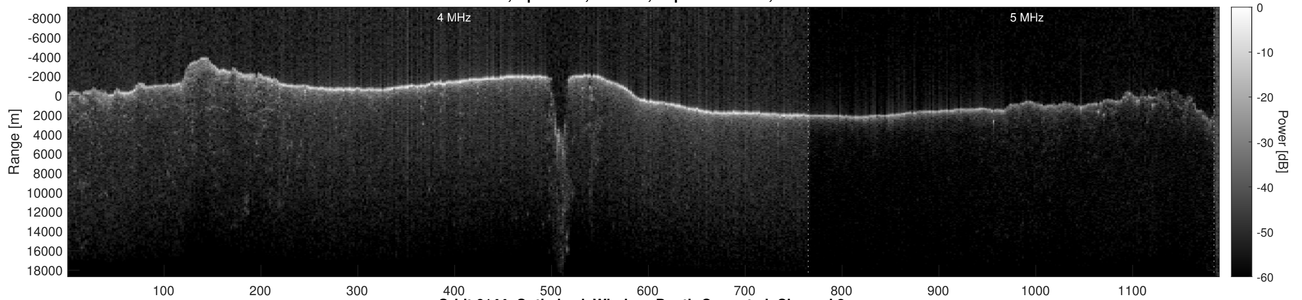
Orbit 6144, Optimized, Window, Depth-Corrected, Channel 2
