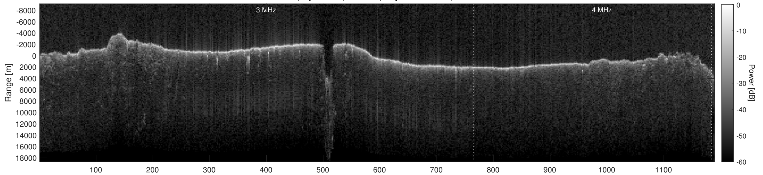
Orbit 6144, Depth-Corrected Cluttergram
