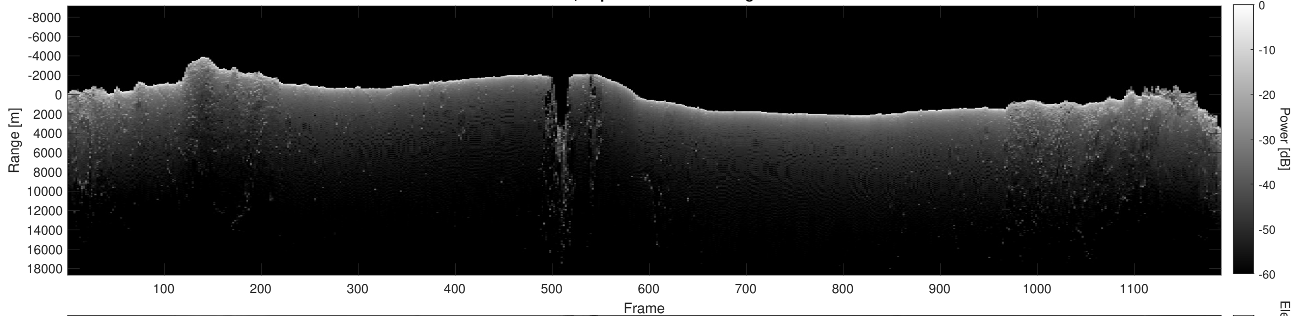
Orbit 6144, Depth-Corrected Cluttergram
