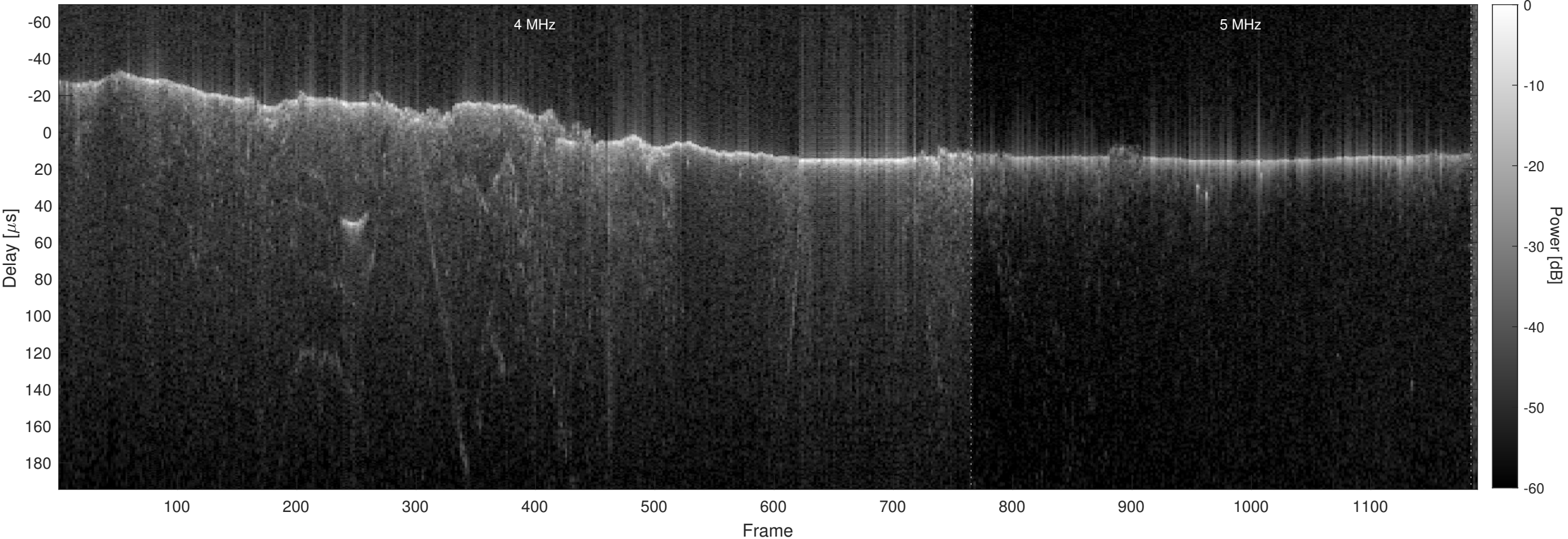
Orbit 6145, Optimized, No Window, Channel 2
