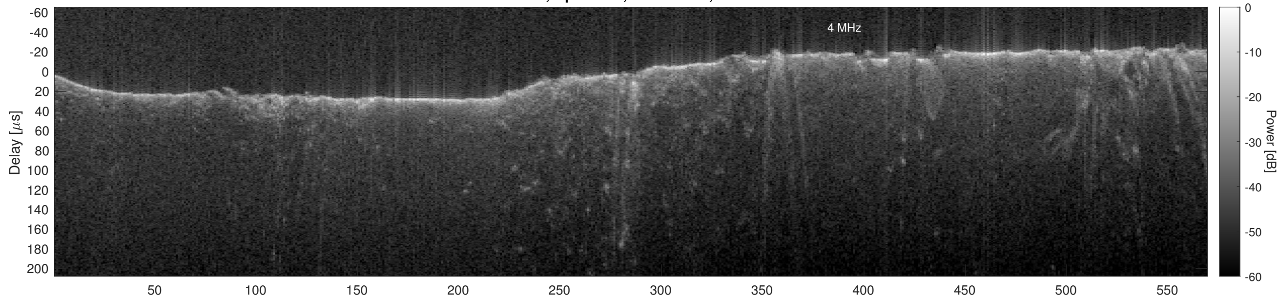
Orbit 6146, Optimized, No Window, Channel 2
