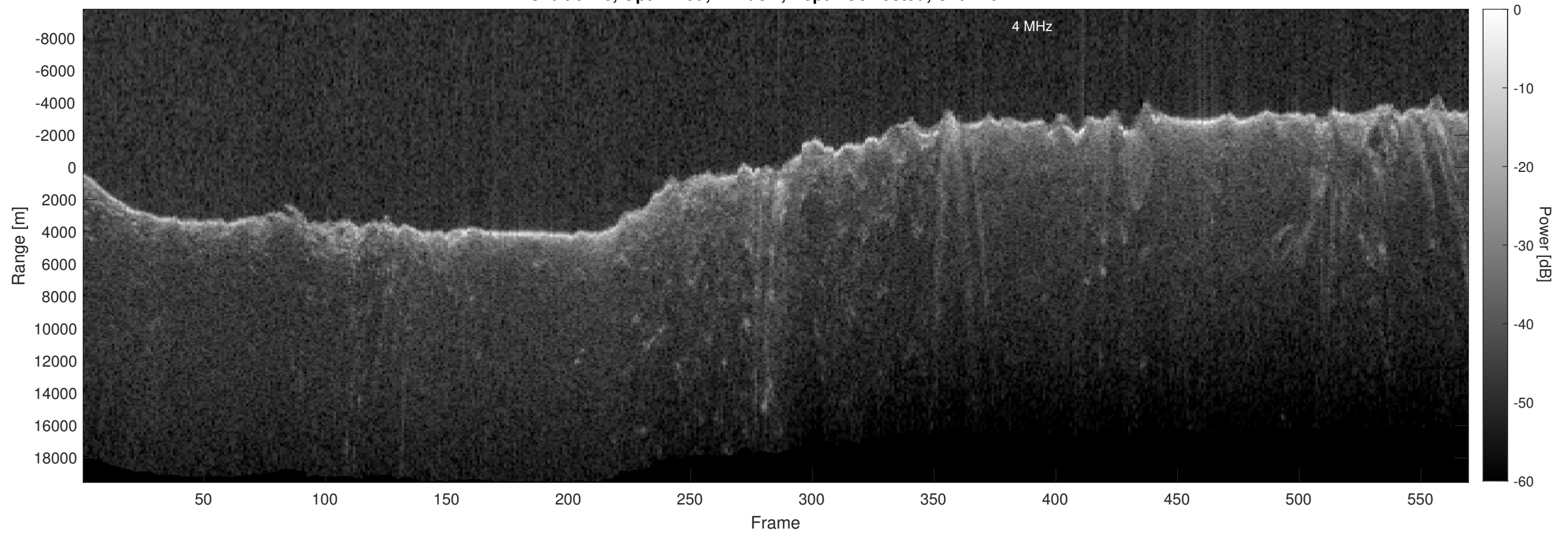
Orbit 6146, Optimized, Window, Depth-Corrected, Channel 2
