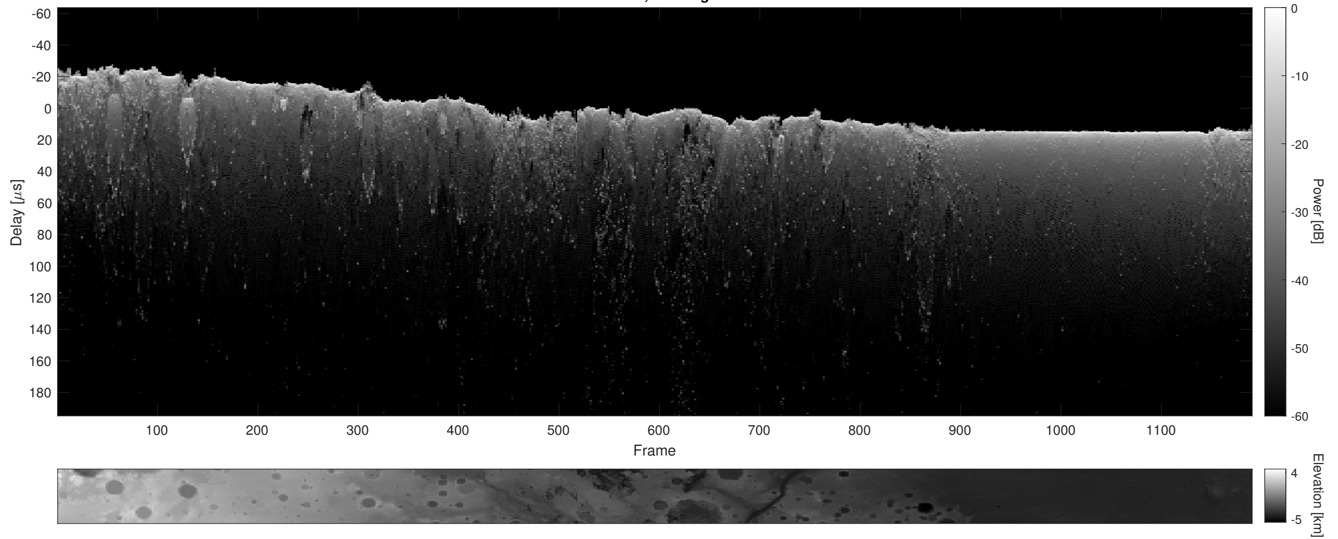
Orbit 6147, Cluttergram
