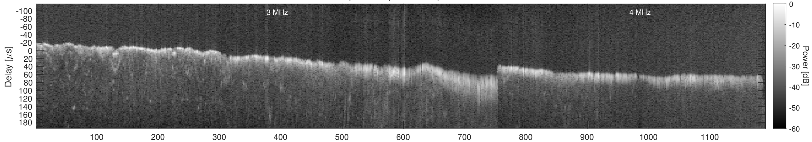
Orbit 6147, Window, Channel 2, Chapman
