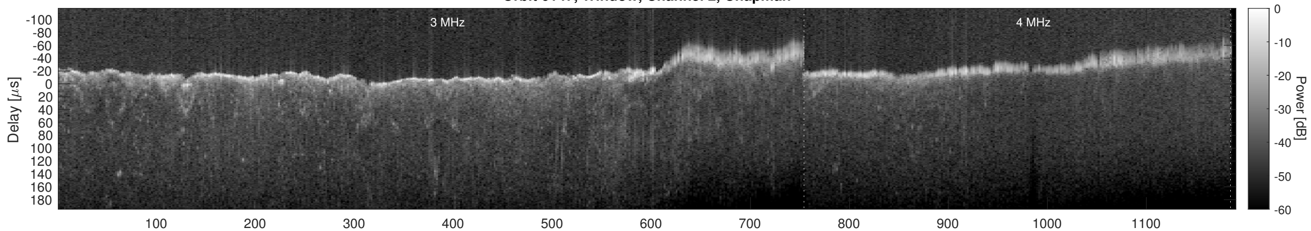
Orbit 6147, Window, Channel 2, Optimized
