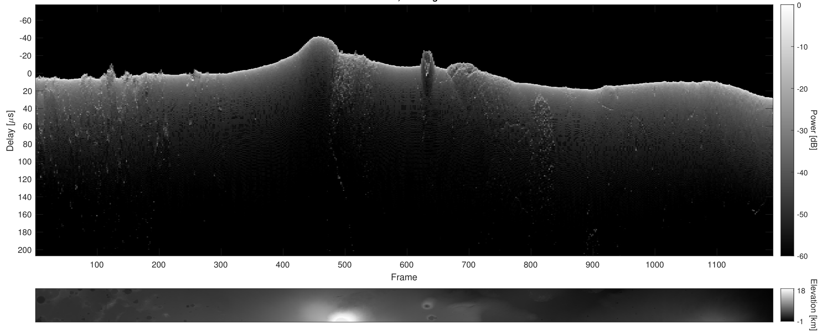
Orbit 6148, Cluttergram
