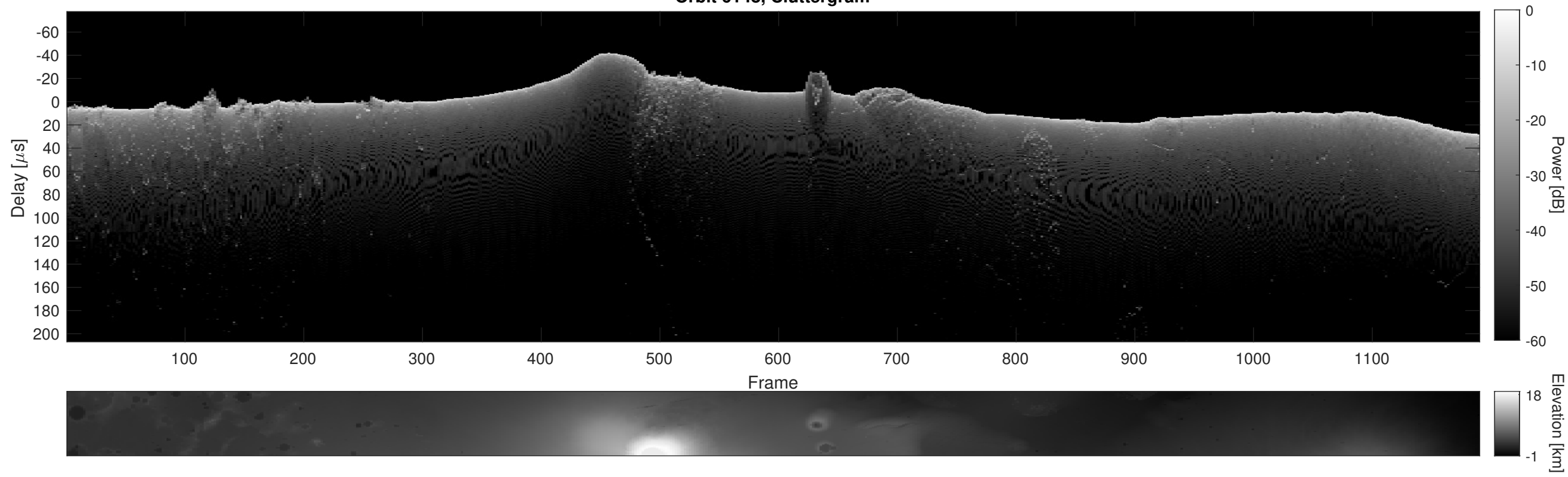
Orbit 6148, Cluttergram
