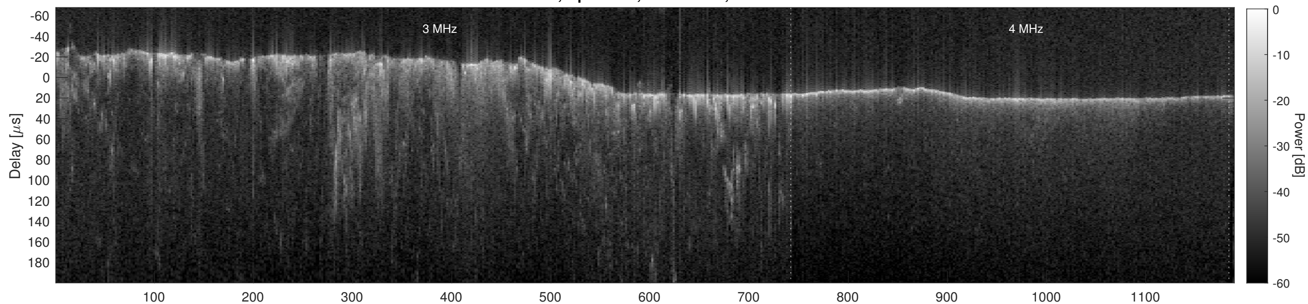
Orbit 6149, Cluttergram
