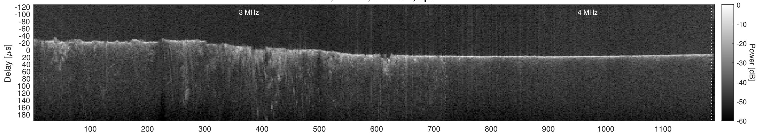
Orbit 6152, Cluttergram
