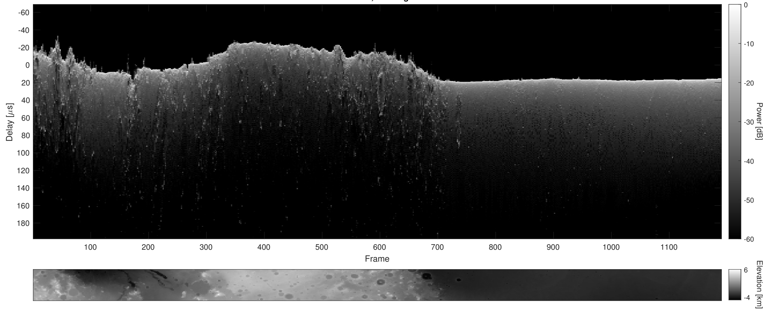
Orbit 6153, Cluttergram
