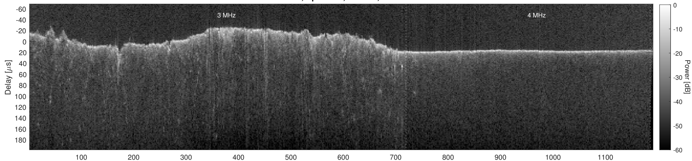
Orbit 6153, Cluttergram
