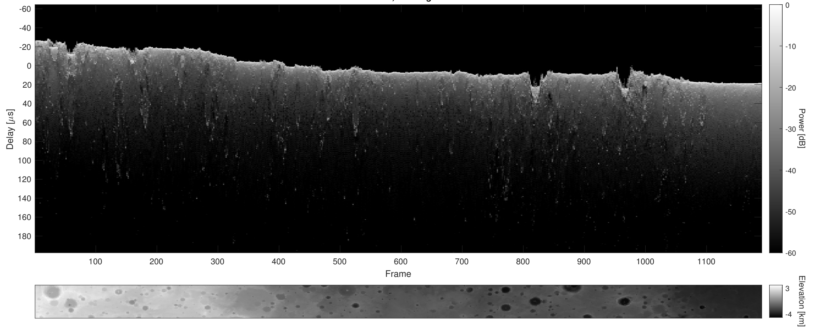
Orbit 6154, Cluttergram
