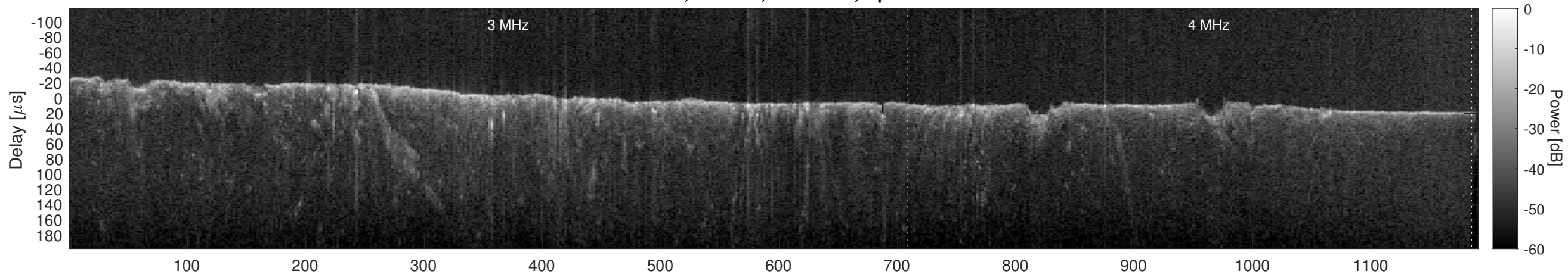
Orbit 6154, Cluttergram
