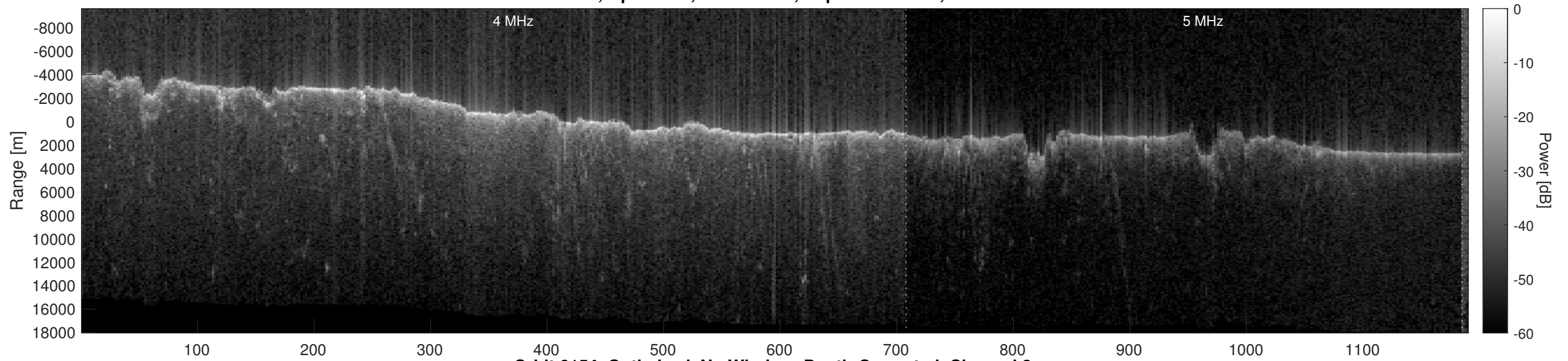
Orbit 6154, Optimized, No Window, Depth-Corrected, Channel 2
