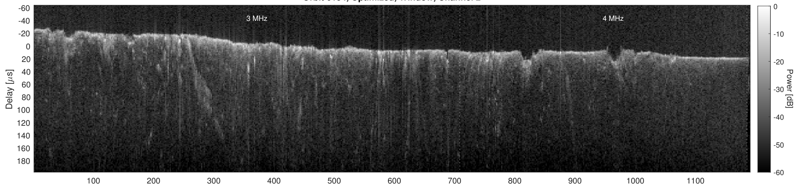
Orbit 6154, Cluttergram
