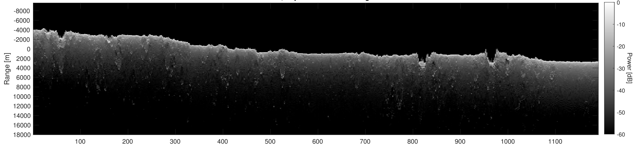
Orbit 6154, Depth-Corrected Cluttergram
