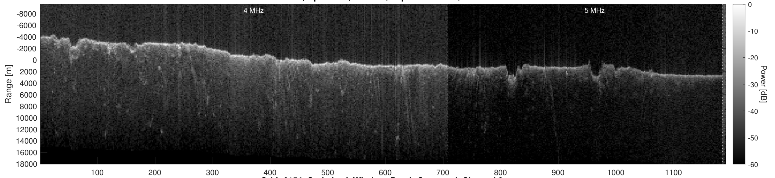
Orbit 6154, Optimized, Window, Depth-Corrected, Channel 2
