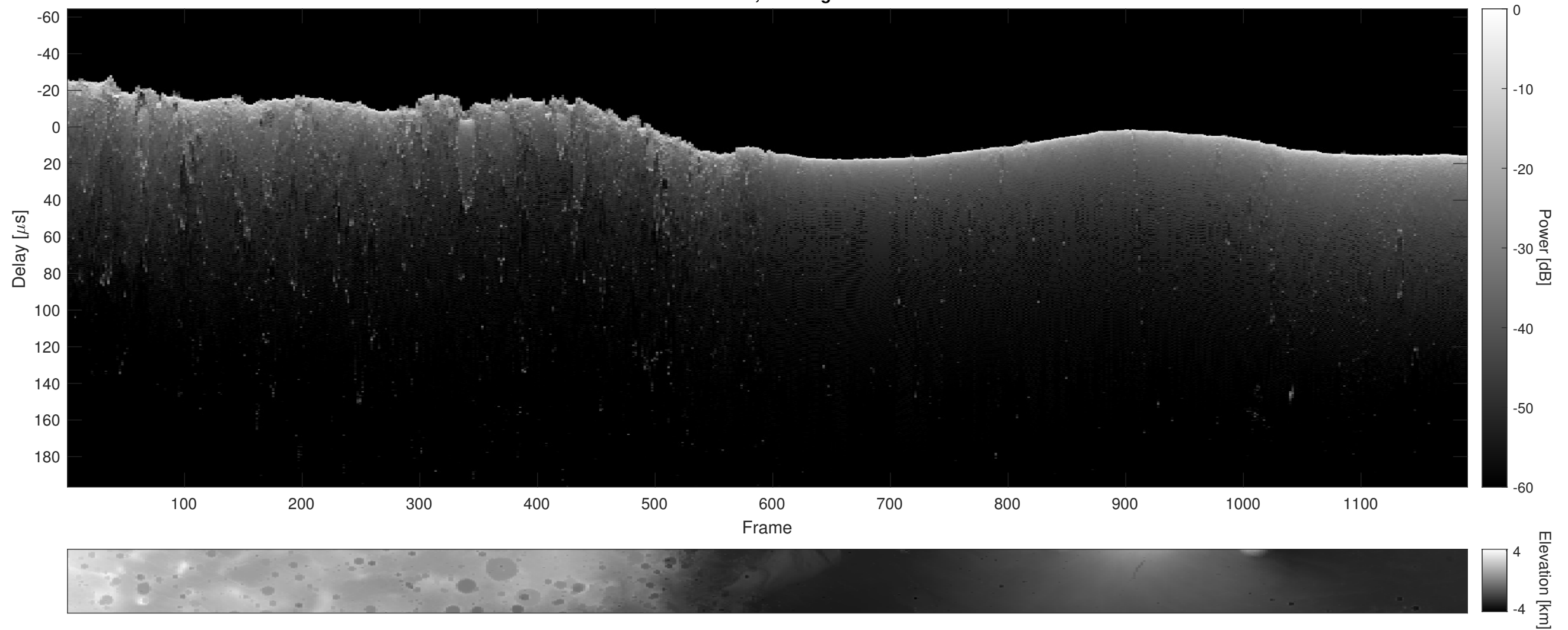
Orbit 6156, Cluttergram
