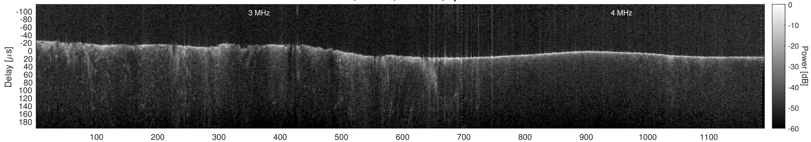
Orbit 6156, Cluttergram
