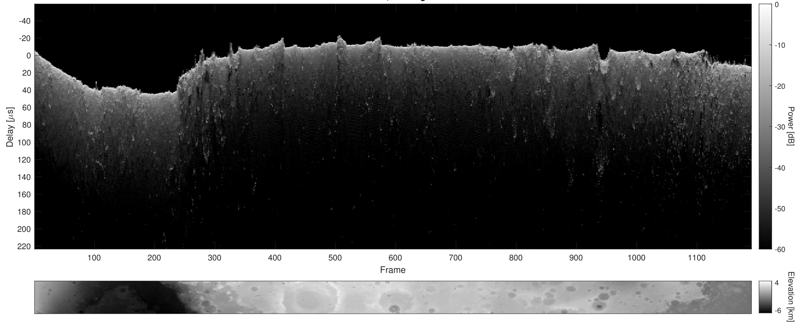
Orbit 6157, Cluttergram
