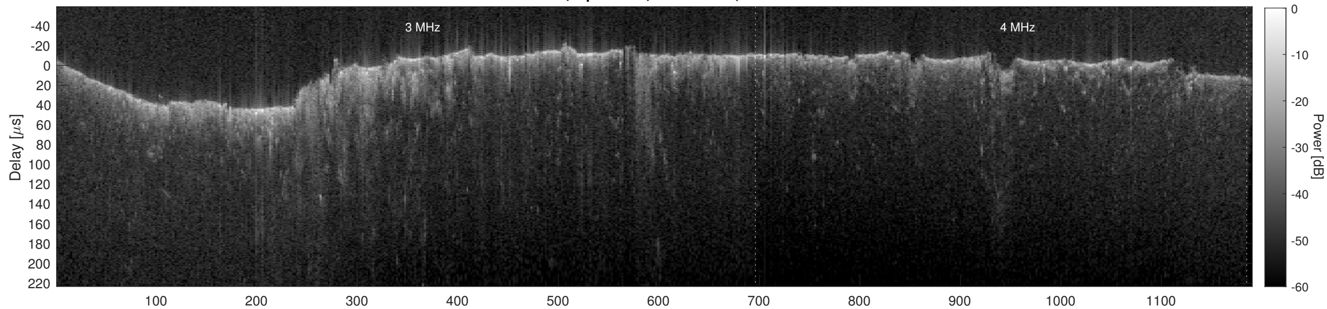
Orbit 6157, Cluttergram
