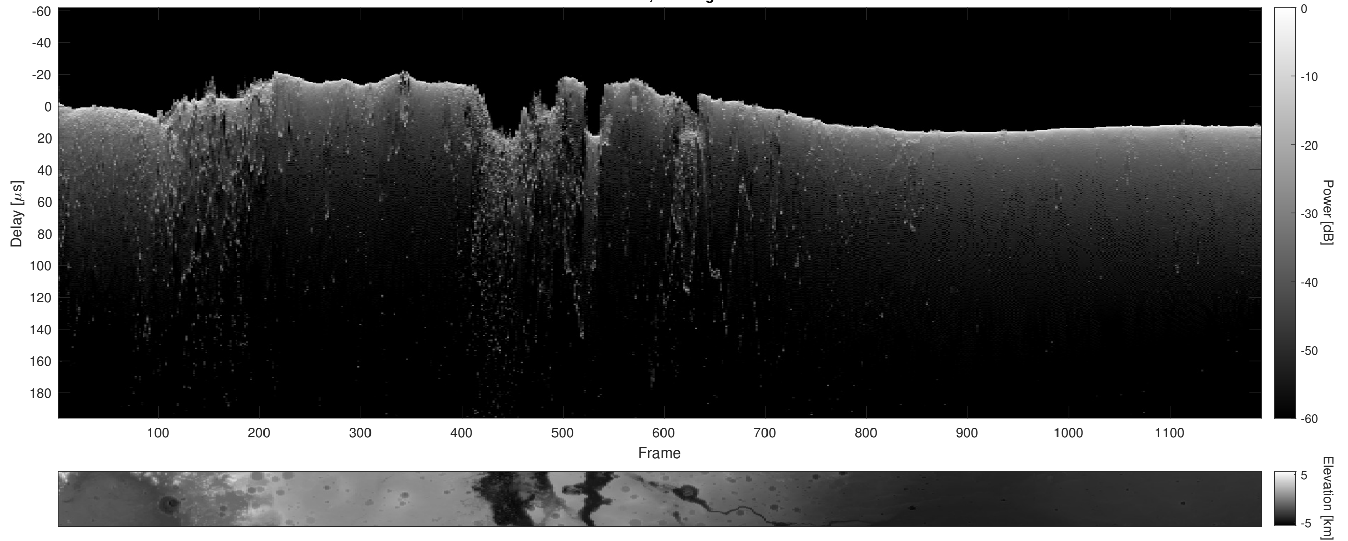
Orbit 6158, Cluttergram
