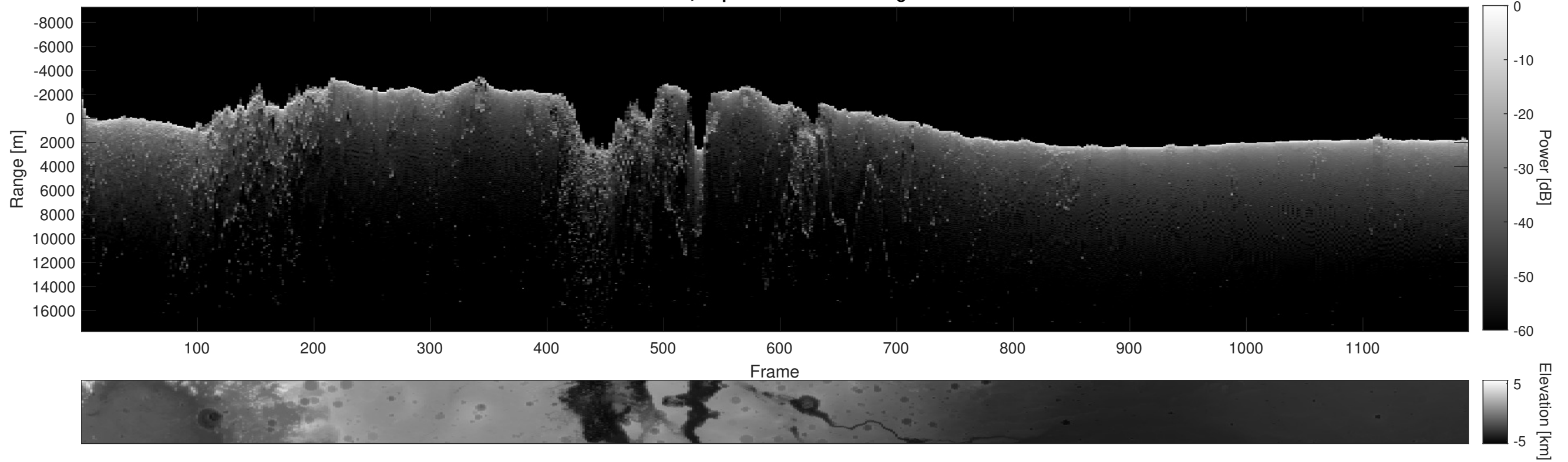
Orbit 6158, Depth-Corrected Cluttergram
