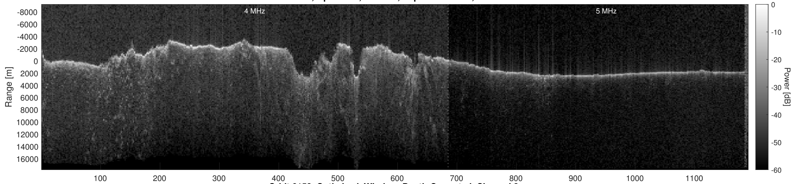
Orbit 6158, Optimized, Window, Depth-Corrected, Channel 2
