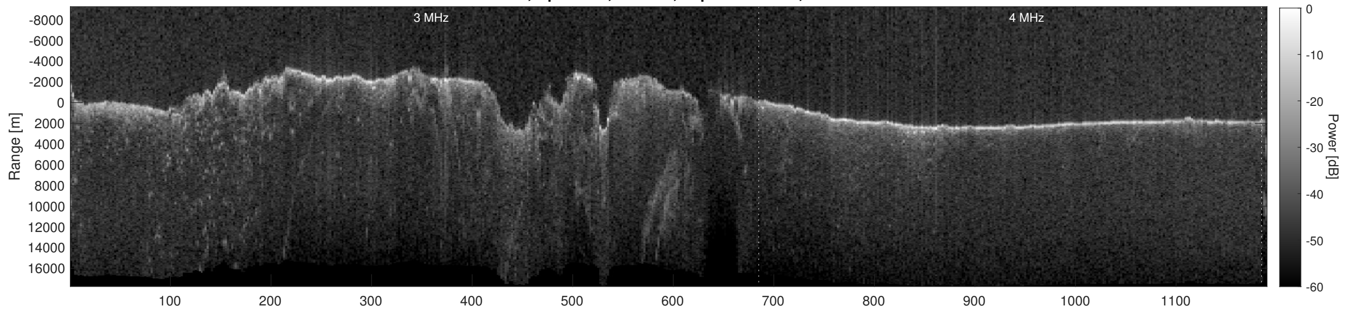
Orbit 6158, Depth-Corrected Cluttergram
