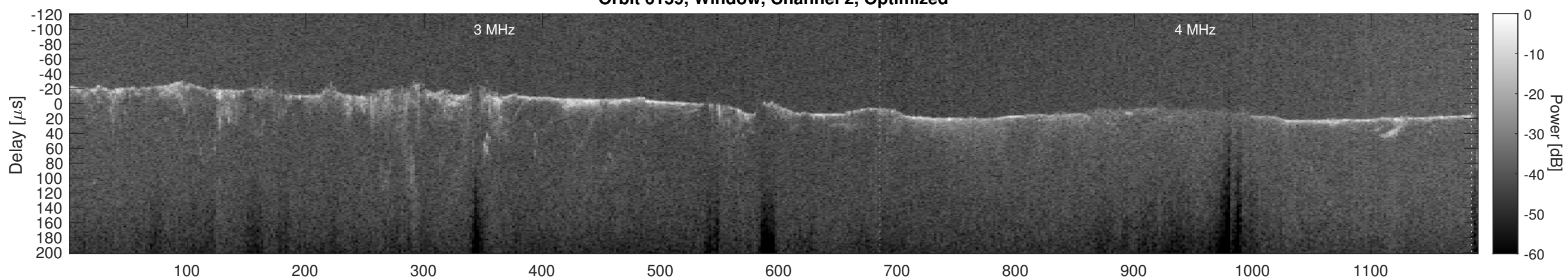
Orbit 6159, Cluttergram
