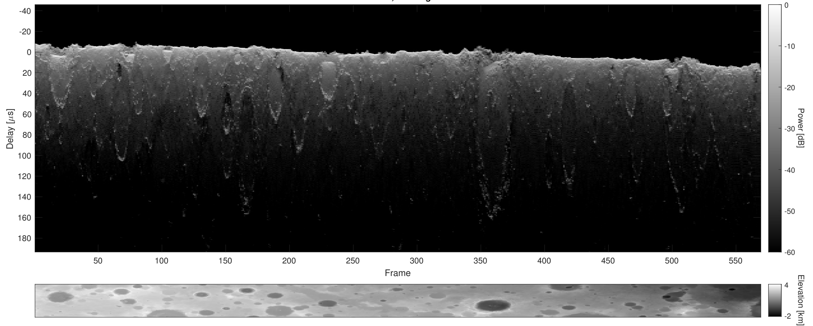
Orbit 6161, Cluttergram
