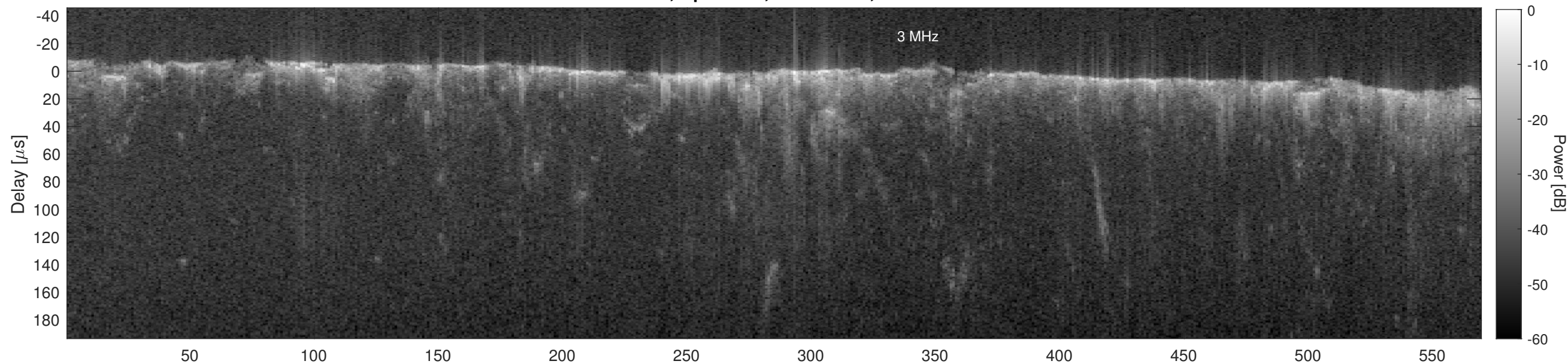
Orbit 6161, Cluttergram
